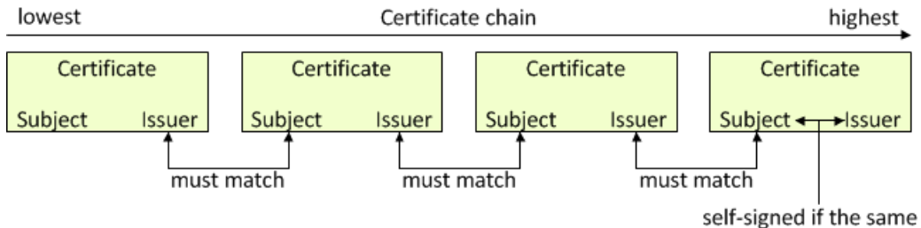
Figure 5-1: Certificate chain
