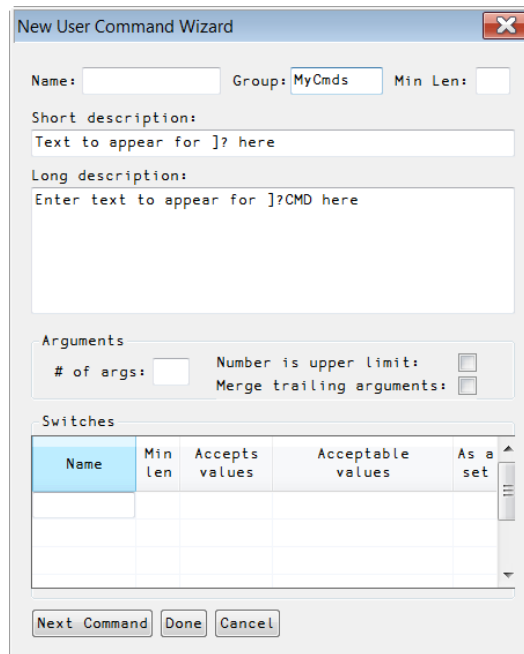
Figure 5-6: The New User Command Wizard
