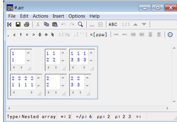
Figure 5-1: The Array Editor
